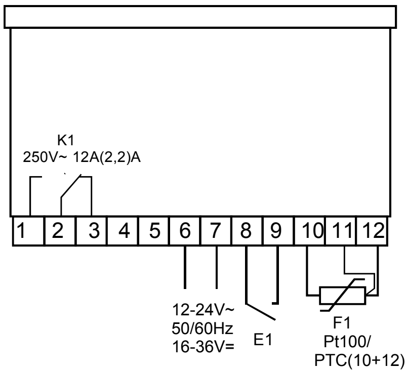
Wiring diagram version 12-24 V~/=
