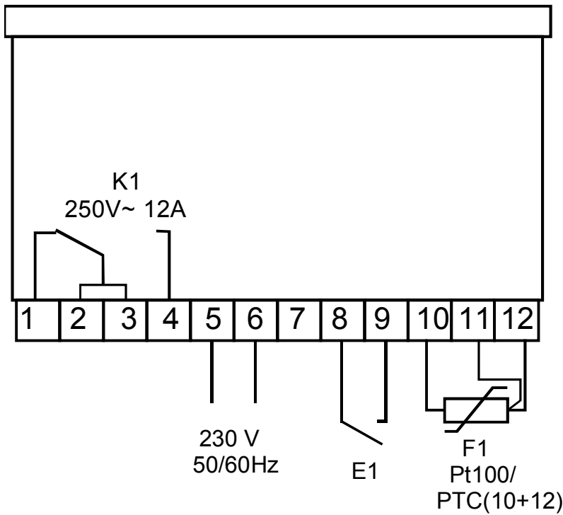
Wiring diagram version 230 V~
