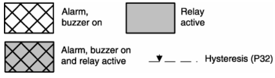
Fig. 5: Boundary alarm, alarm contact invers A30=4 limits relative A30=5 limits absolute
